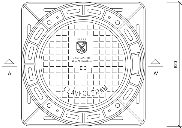
Tapa circular
