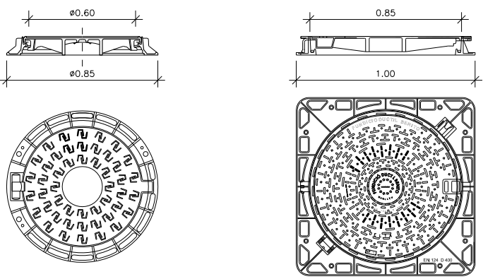
DETALLS TAPES REGISTRE ESCALA 1/30
